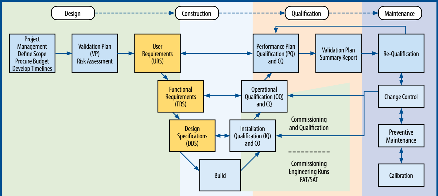
The ISPE general V-model
